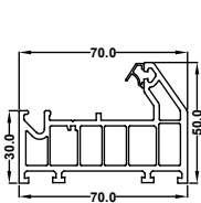
EWS 7001 50mm Door low threshold
