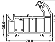
EWS 7720 55mm Standard window outer frame
