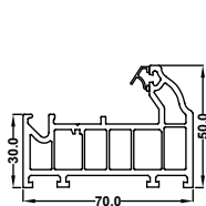
EWS 7701 50mm Door low threshold
