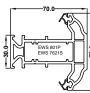
EWS 801P EWS 7621S Small transom internal glazed
