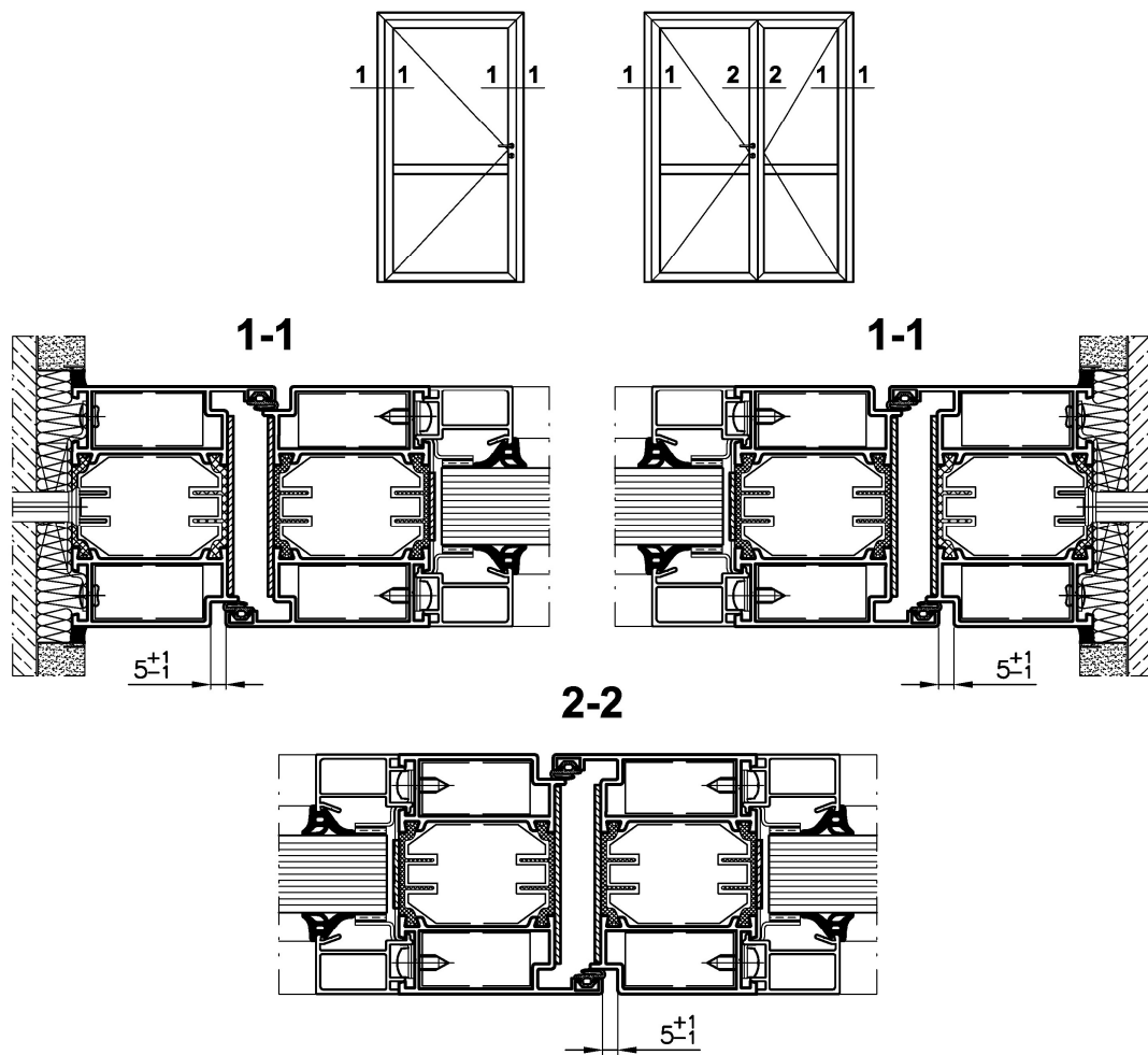
Fig. 29 Doors with standard closing devices – permissible clearances between frame and leaf, and between leaves
