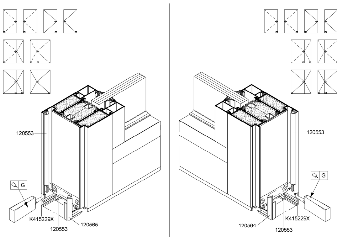
Fig. 36 Sealing of lower corners of the active and inactive leaf (leaf frame lower transom made of crosspiece profile)
