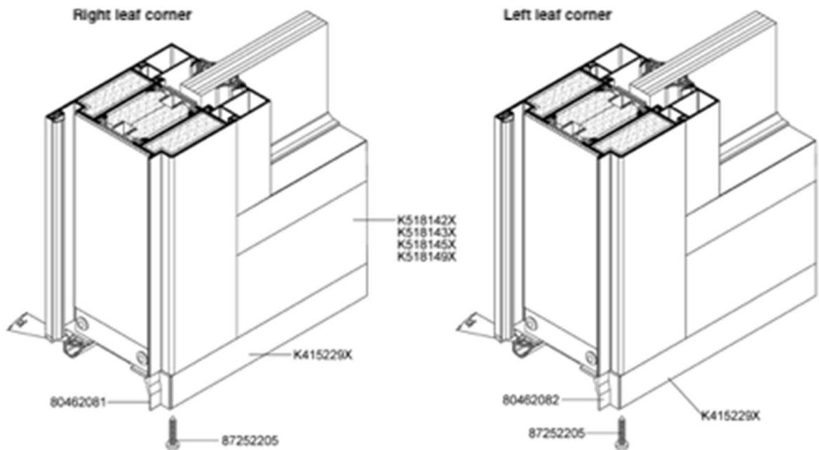
Fig. 35 Sealing of lower corners of the inactive leaf (leaf frame lower transom made of crosspiece profile)
