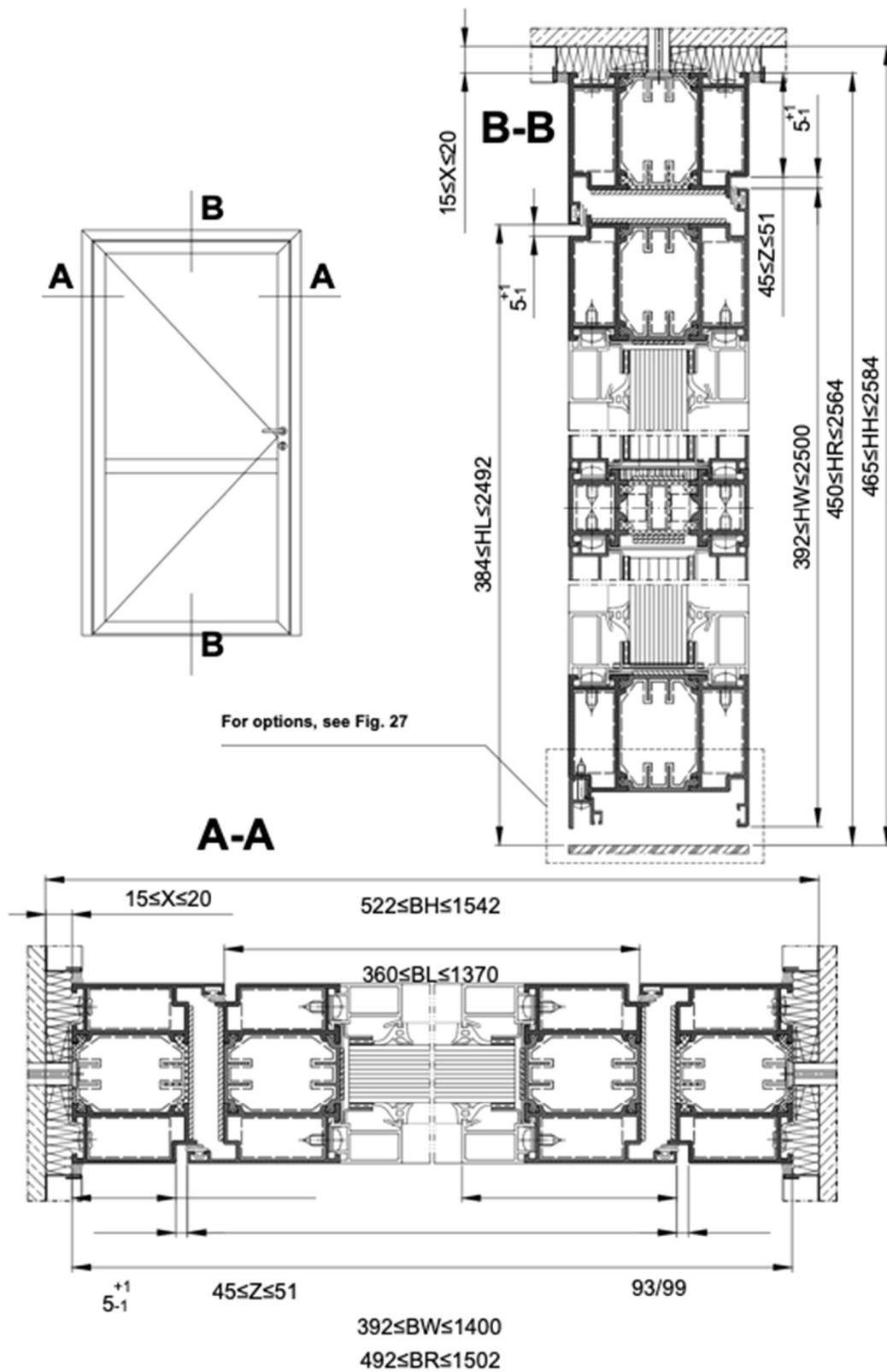
Fig. 13 Dimensional specification of the installation of single door MB-78 EI90
