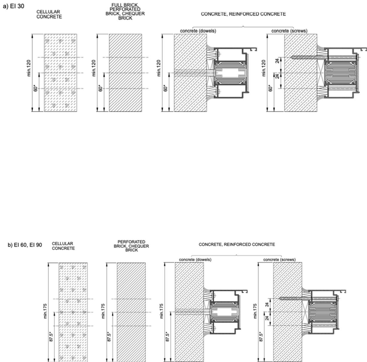
Fig.3. Recommended distance of dowels and screws from the edge of the frame for walls made of various building materials (required wall density: min. 650kg/m 3 )
