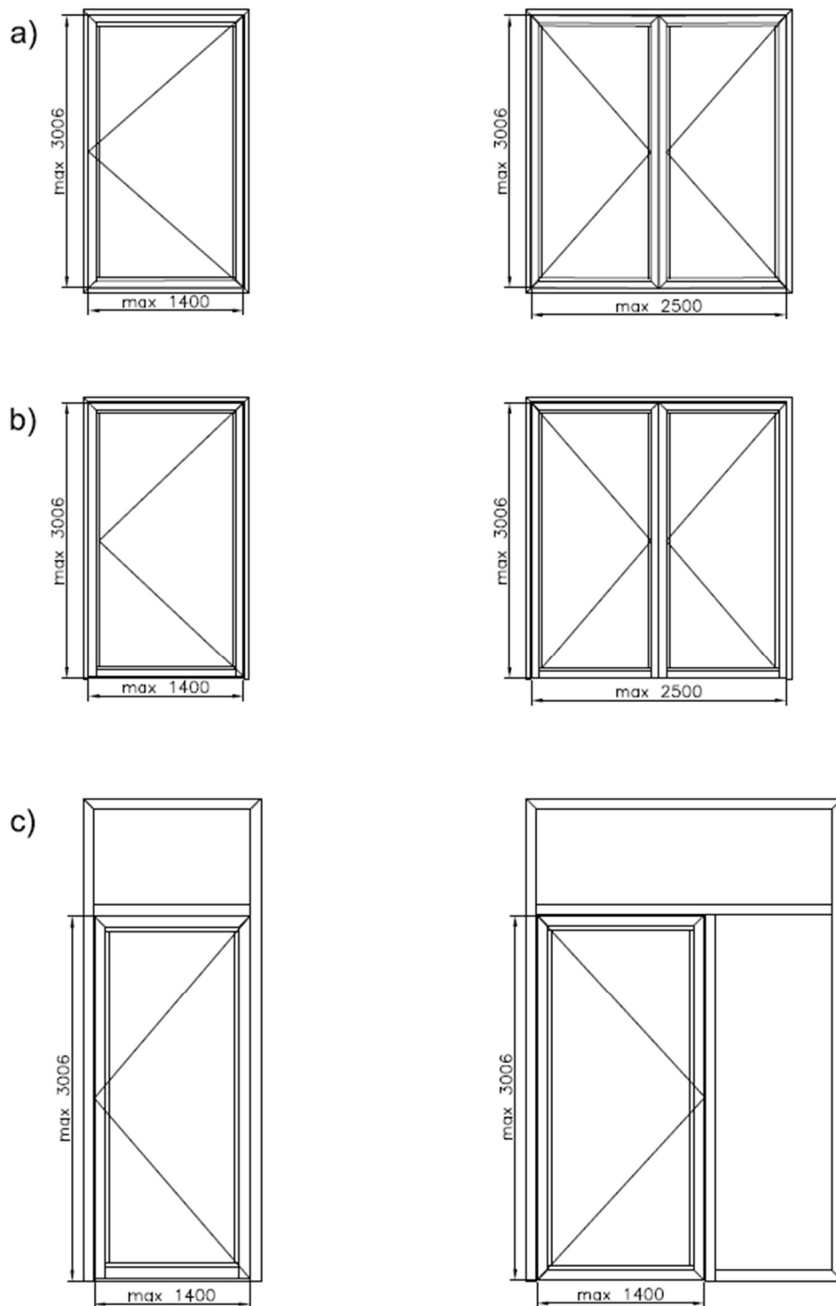
Fig. 5 Types of fire constructions rated EI60 and leaf maximum dimensions: a) technical windows; b) doors; c) door systems
