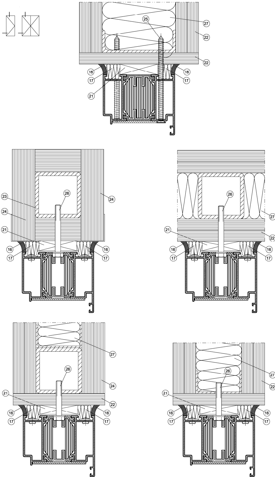
Fig. 21 Sealing variants for frame connections in doors, technical windows and door system frames rated EI30, embedded in framed flexible walls cladded with plasterboards
