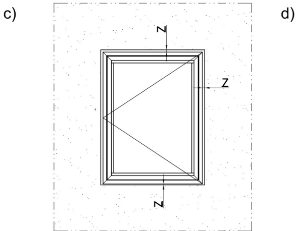
Fig.1. Standard 'Z' clearance between wall frame and fire-rated door frame or fire-rated technical window frame
