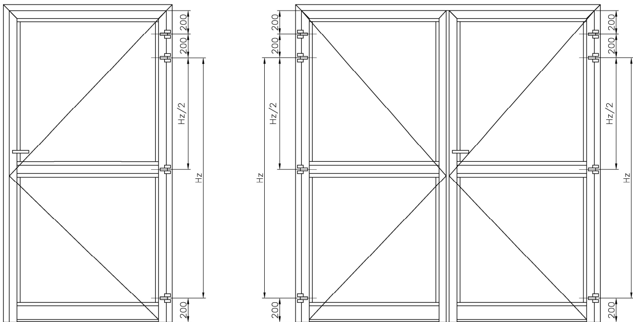
Fig. 37 Arrangement of hinges
