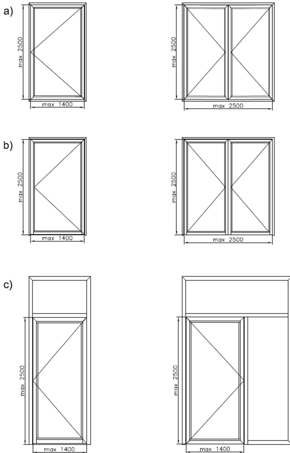
Fig. 6 Types of fire constructions rated EI90 and leaf maximum dimensions: a) technical windows; b) doors; c) door systems
