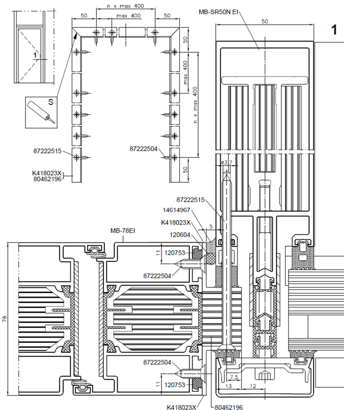
Fig. 25 Installation of door frame in ALUPROF MB-SR50N EI filling type curtain wall
