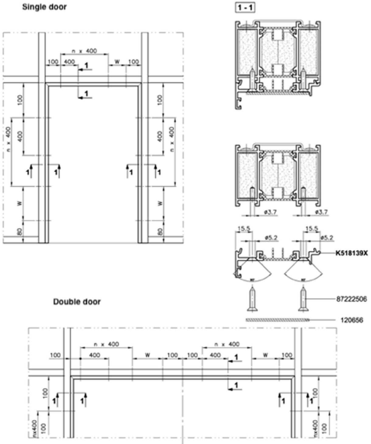
Fig. 31 Installation of edging strip K518139X
