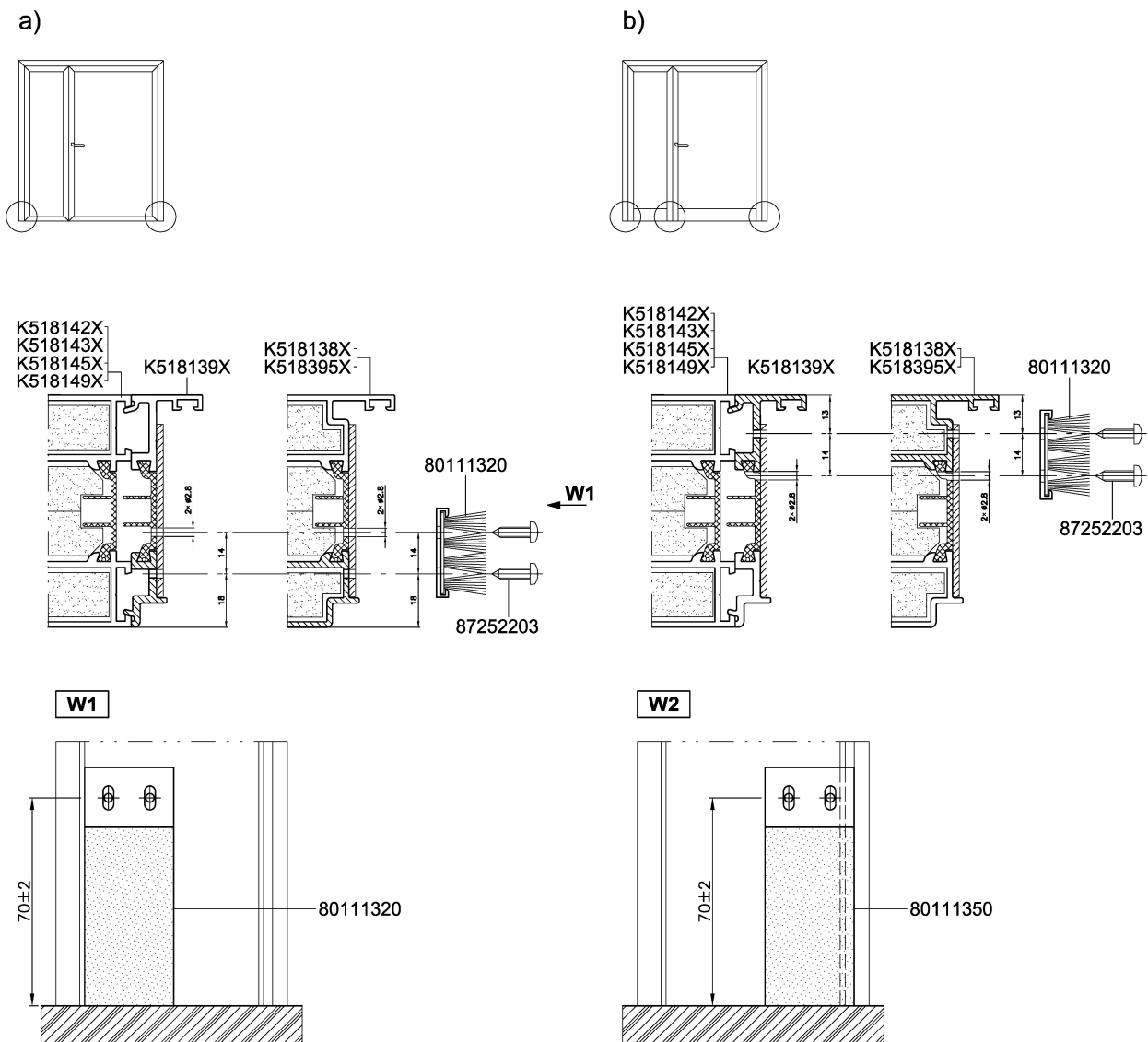
Fig. 33 Door stop sealing (applies to all fire resistance classes):
