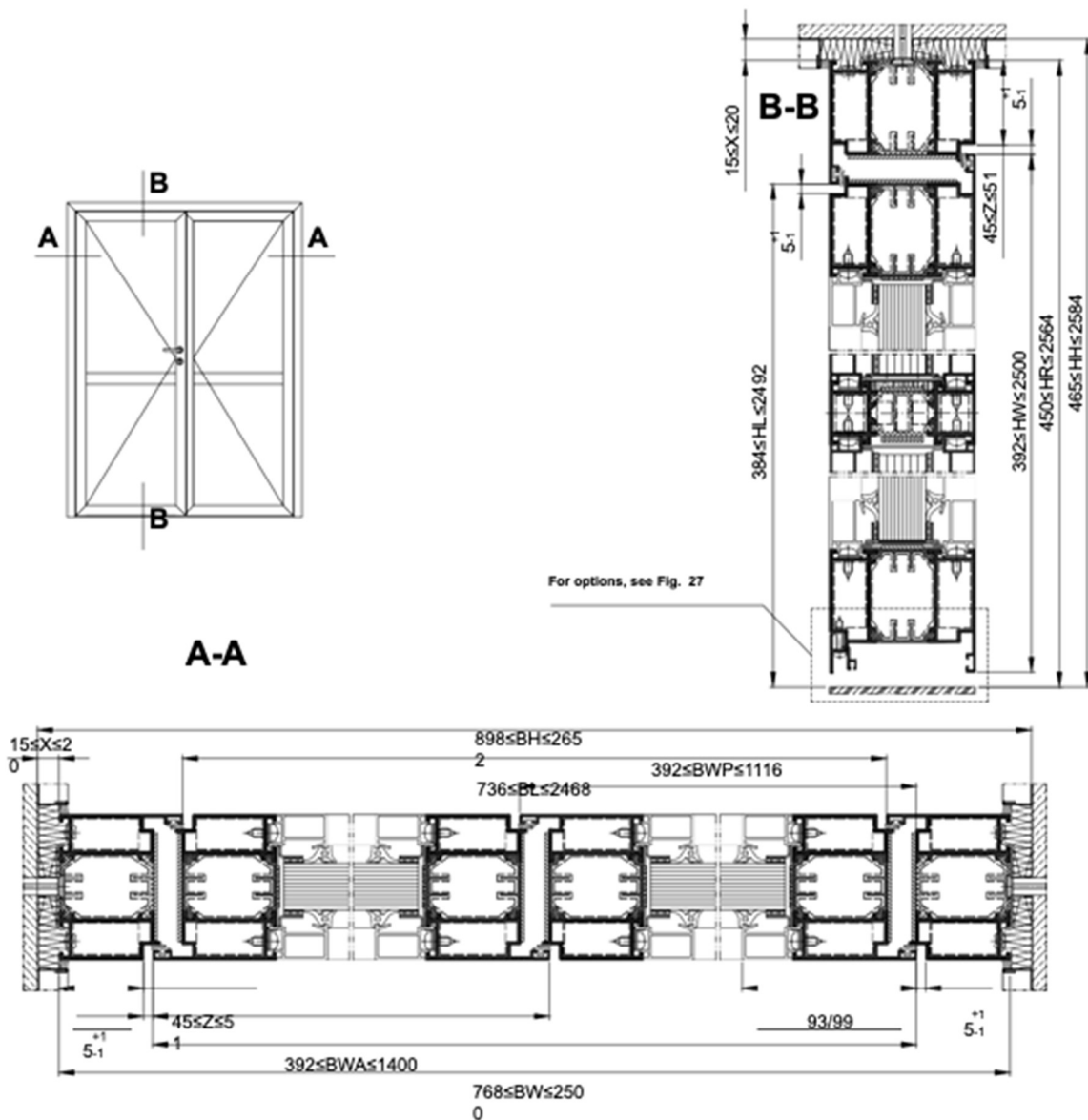
Fig. 15 Dimensional specification of the installation of single door MB-78 EI90
