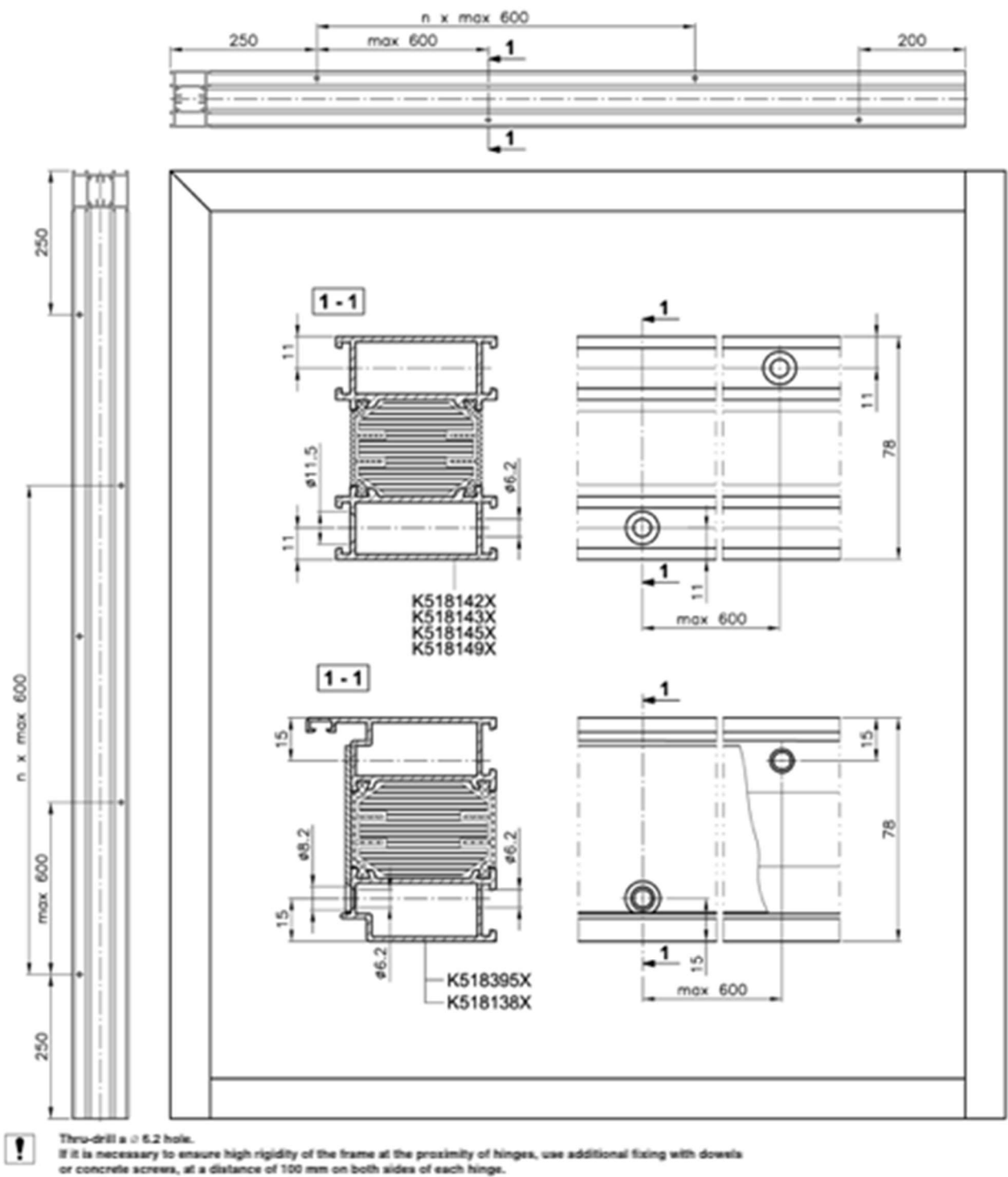
Fig. 17 Preparation of frames for fixing to the building structure using concrete screws
