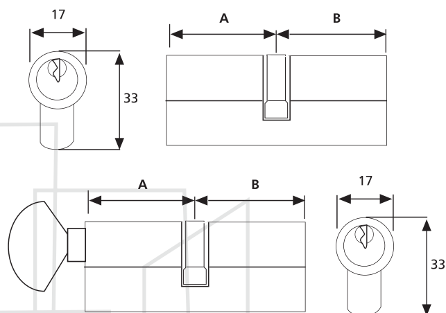
Economy Euro Profile Cylinder
